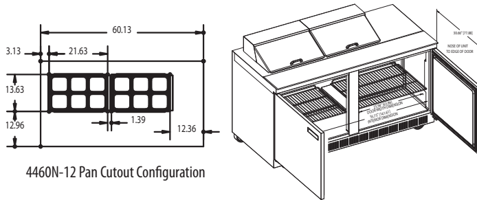
4460N-12 ISO View
